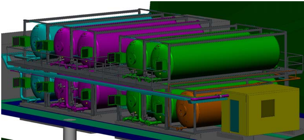
Design model aircraft deicing fluid storage tank farm
